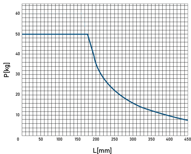
HORIZONTAL LOAD
