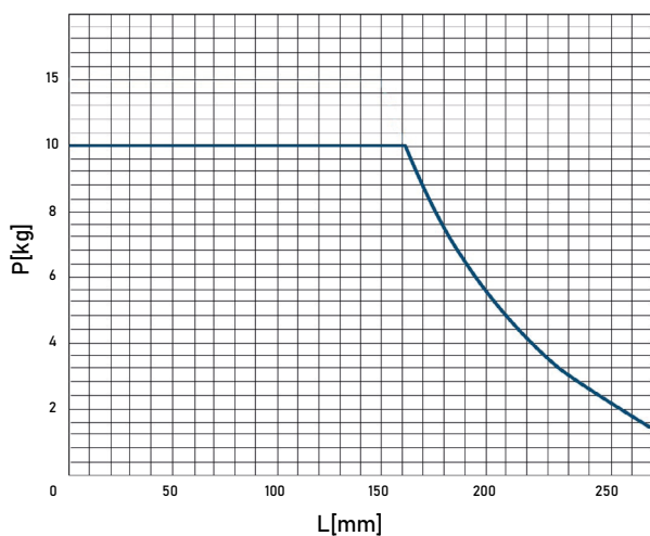
VERTICAL LOAD
